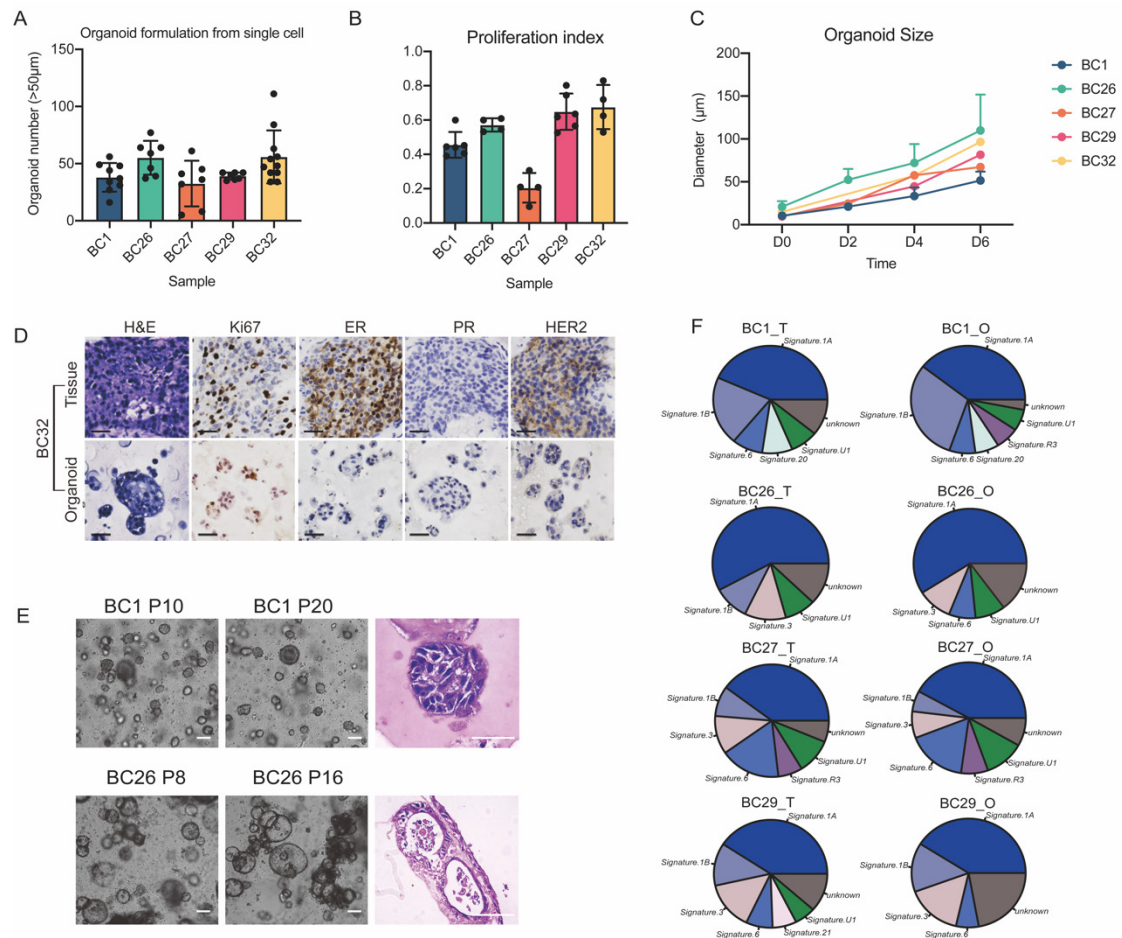
Fig. S1. PDOs maintain tumor heterogeneity. (A) Number of organoid formulations. Error bars: \pm s.d, n \geq 6 . (B) Proliferation index of each BC-PDO. Error bars: \pm s.d, n \geq 4 . (C) Diameter size of PDOs from day0 (D0) to day6 (D6). Error bars: \pm s.d, n=4 . (D) H&E and IHC staining displayed molecular features. Scale bar: 100 \mu m. (E) PDOs maintained histological features after long-term passages. Scale bar: 100 \mu m. (F) PDOs maintained genomic signatures after long-term passages.
